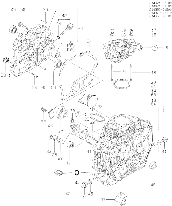
Fig.1. CYLINDER BLOCK
