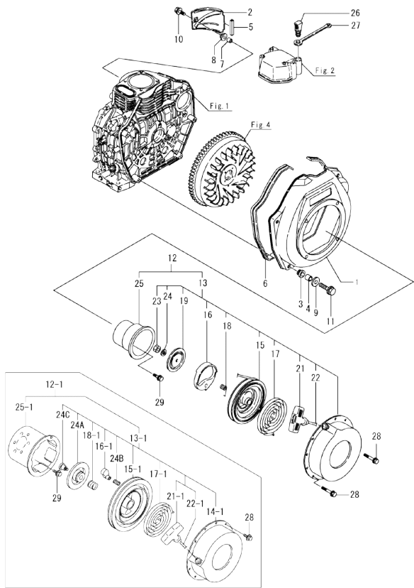
Fig.6. COOLING & STARTING DEVICE
