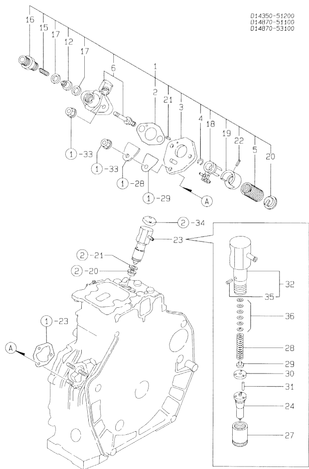
Fig.7. FUEL INJECTION PUMP
