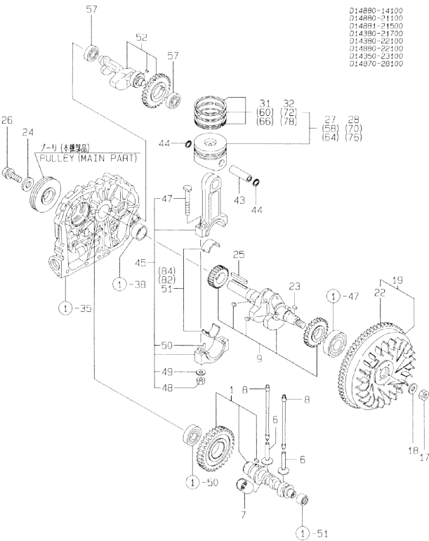
Fig.4. CRANKSHAFT,PISTON & CAMSHAFT
